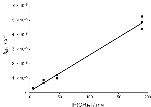
Figure 2. Plot of k_{\text{obs}} ( \text{s}^{-1} ) for approach to equilibrium of cis / trans - P,P - 5 versus [\text{P}(\text{O}-o\text{-tolyl})_3] from three separate experiments. For [\text{P}(\text{O}-o\text{-tolyl})_3] = 5.6, 23, and 46 \text{ mM} , the data points for the separate experiments overlap.
