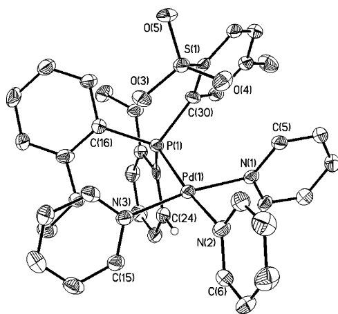
Figure 1. Molecular structure of the cation of [\{\text{PO-OMe}\}\text{Pd}(\text{py})_3][\text{SbF}_6] ( 4 ). Hydrogen atoms except H(24) are omitted. Bond lengths [Å]: Pd(1)–N(1) 2.051(6), Pd(1)–N(2) 2.096(6), Pd(1)–N(3) 2.028(6), Pd(1)–P(1) 2.291(1), Pd(1)–O(3) 3.066(5), Pd(1)–H(24) 2.83.
