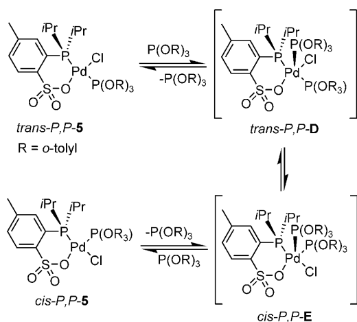
Scheme 3. Proposed mechanism for the \text{P}(\text{O}-o\text{-tolyl})_3 -catalyzed isomerization of 5 .
