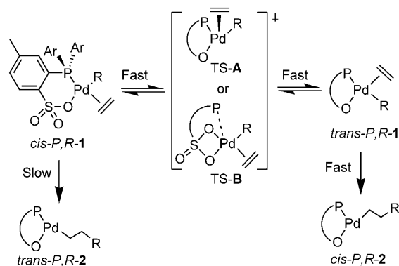
Scheme 1. Proposed chain-growth mechanism for [\{\text{PO}\}\text{PdR}] catalysts.
