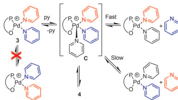
Scheme 2. Pyridine exchange mechanism for 3 . \widehat{\text{PO}} = \{\text{PO-OMe}\} .
